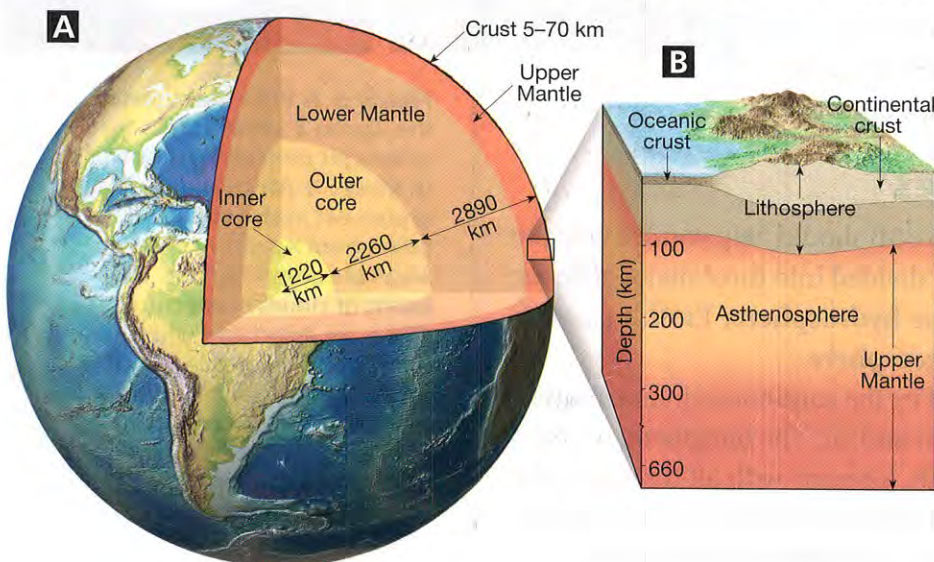
Figure 6 A On this diagram, the inner core, outer core, and mantle are drawn to scale but the thickness of the crust is exaggerated by about 5 times. B There are two types of crust—oceanic and continental. The lithosphere is made up of the crust and upper mantle. Below the lithosphere are the asthenosphere and the lower mantle.
