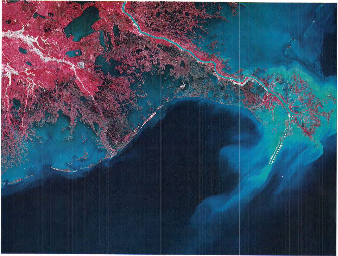
Figure 17 Satellite Image of the Mississippi River Delta Moving sediment (light blue) indicates current patterns. Red shows vegetation.
